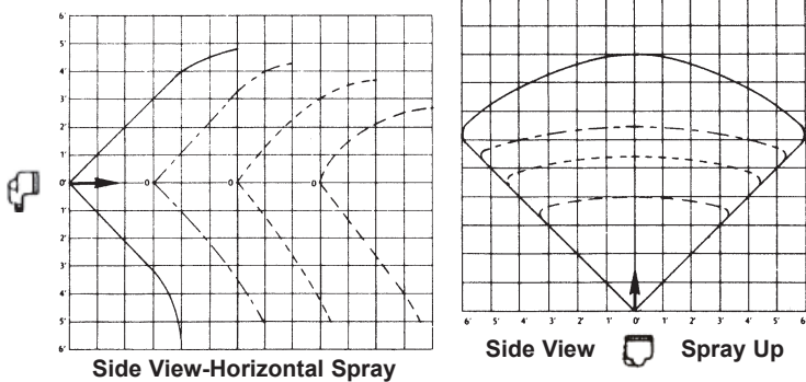
Side View-Horizontal Spray
