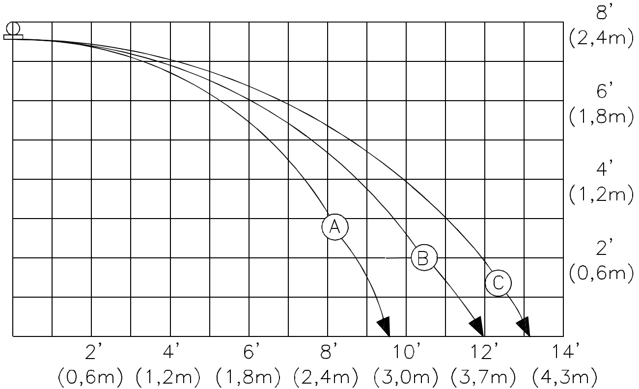
Typical profile of one half of the spray pattern produced by a Viking Micromatic® Model N-2 1/2" (15 mm) Pendent Sprinkler SIN VK132 (Nominal K-Factor = 5.6 U.S.)
