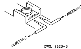
FIG. 6 SWITCH TERMINAL CONNECTIONS CLAMPING PLATE TERMINAL
