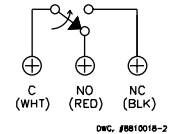
FIG. 6 SWITCH TERMINAL CONNECTIONS CLAMPING PLATE TERMINAL
